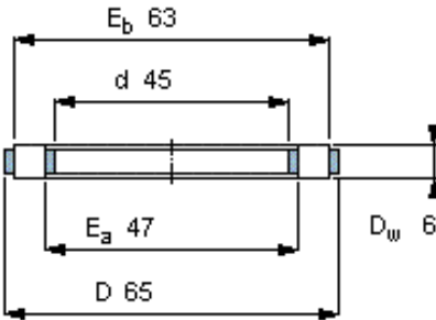
Roller and cage thrust assembly
