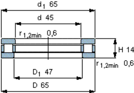
Complete bearing
